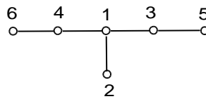
Figure 1. The graph G(\mathbf{A}) of sign pattern \mathbf{A}
