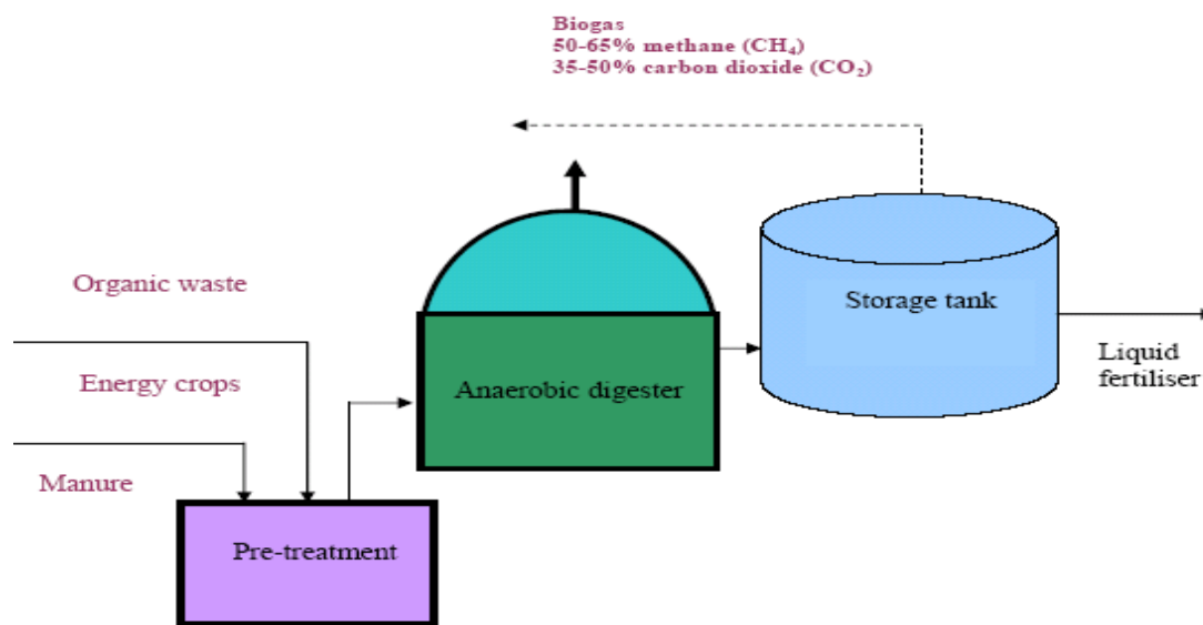
Figure 2. General schematic of an agricultural biogas plant [3]
