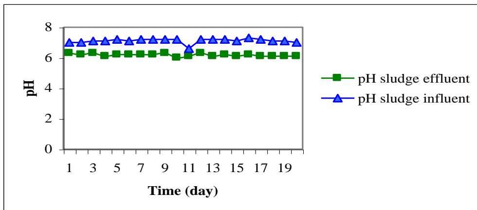
Figure 6. pH sludge before and after treatment in the digester [24]
