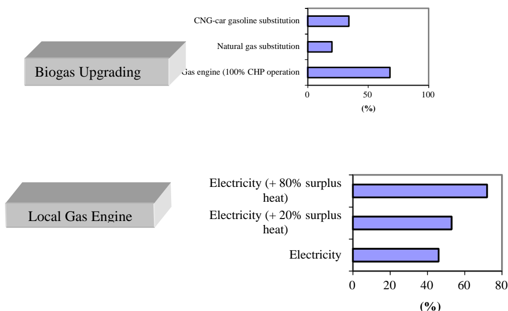
Figure 4. Greenhouse gas emissions savings for different biogas utilisation pathways in comparison to fossil energy production [17]
