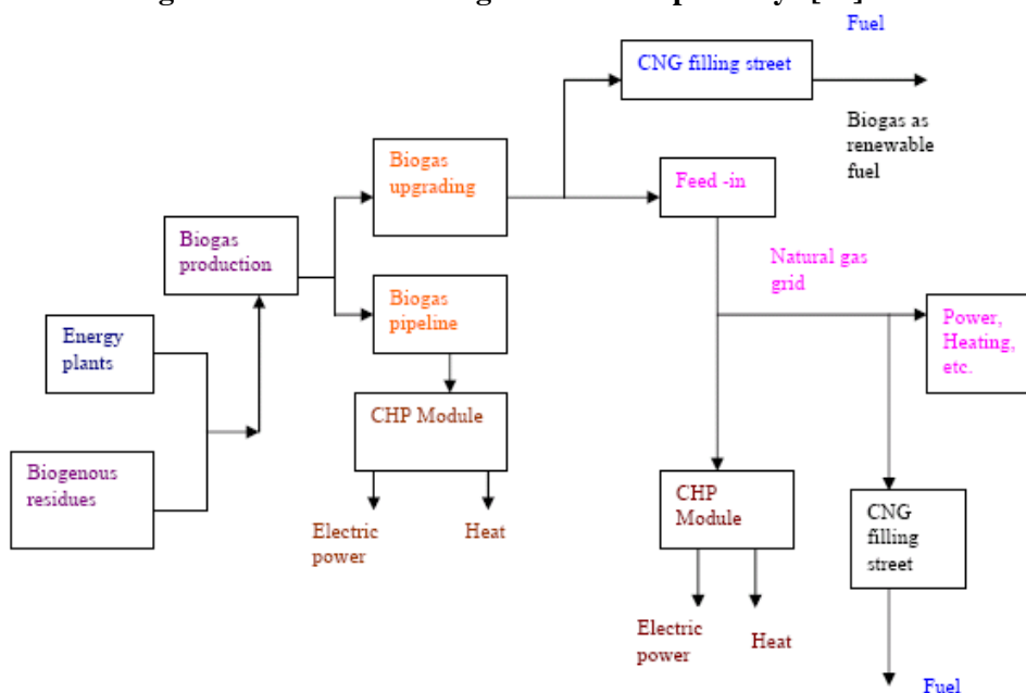
Figure 3. Overview of biogas utilisation pathways [17]
